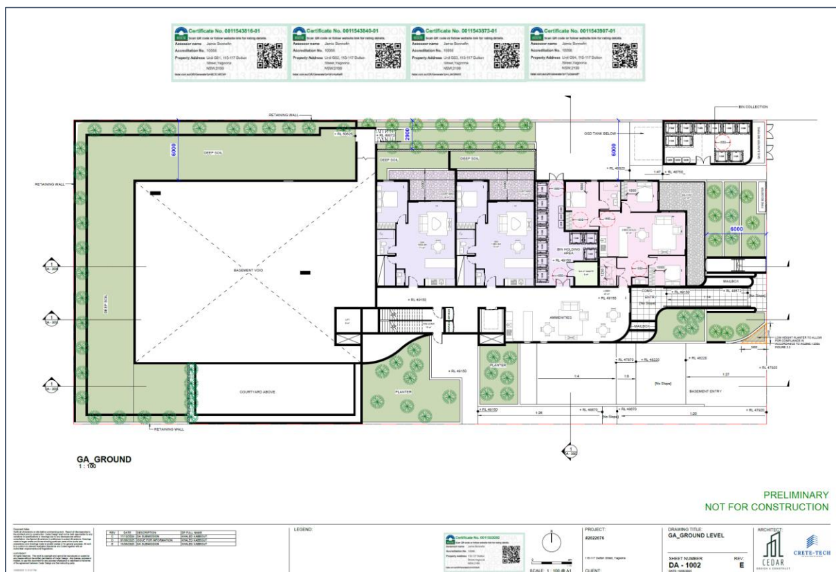
Figure 3.1 – Proposed ground floor plan (Source: Cedar Design & Construct)
